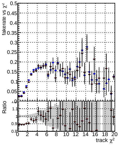
Fake rate vs. DOM TT original DOM TT initOnly DOM TT FWD8 PU
