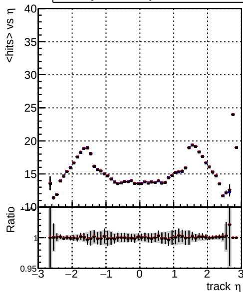
mean hits vs \eta — DQM_TT__original — DQM_TT__initOnlyFWD0_PU — DQM_TT__initOnlyFWD0_PU
