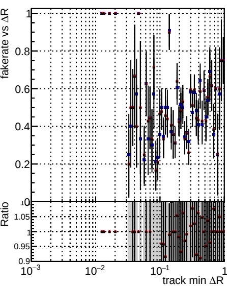
Legend: DQM TT original (black line with blue dots), DQM TT initOnlyFWD0_PU (red line with red dots), DQM TT initOnlyFWD0_PU (black line with black dots)
