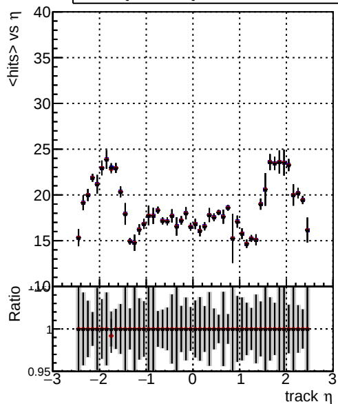
mean hits vs \eta — DQM_TT_original — DQM_TT_detQ0_PU — DQM_TT_detQ1_PU
