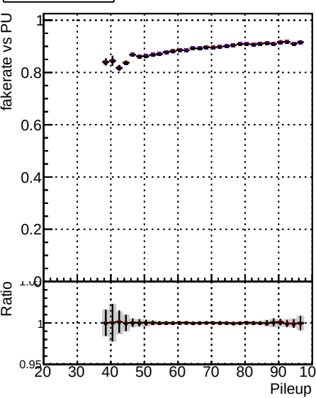
Fake rate vs Pileup
