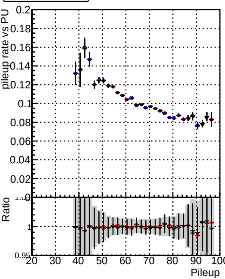
Pileup rate vs Pileup
