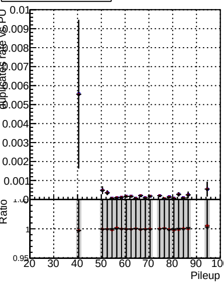
Duplicates Rate vs Pileup
