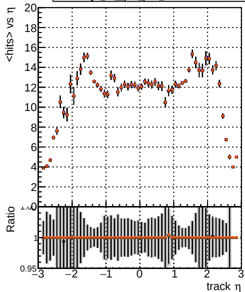
mean hits /data2/legianni/pareto-opt/restart/CMSSW_14_0_5/src/MIV-plot/DQM_TT_original_PU DQM_TT pLF pt09 1PU DQM_TT pLF pt09 2PU DQM_TT pLF pt09 3PU
