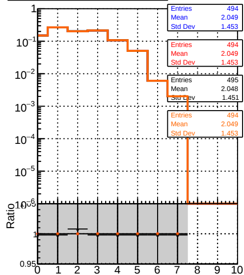
mean hits vs \eta Legend: /data2/legianni/pareto-opt/restart/CMSSW_14_0_5/src/MIV-plot/DQM_TT_original_PU - DQM_TT_pLF_pt09_1PU (blue line with dots) - DQM_TT_pLF_pt09_2PU (red line with dots) - DQM_TT_pLF_pt09_3PU (orange line with dots)
