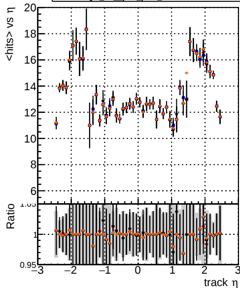
mean hit /data2/legianni/pareto-opt/restart/CMSSW_14_0_5/src/MIV-plot/DQM_TT_original_PU DQM_TT_pLF_pt09_1PU DQM_TT_pLF_pt09_2PU DQM_TT_pLF_pt09_3PU
