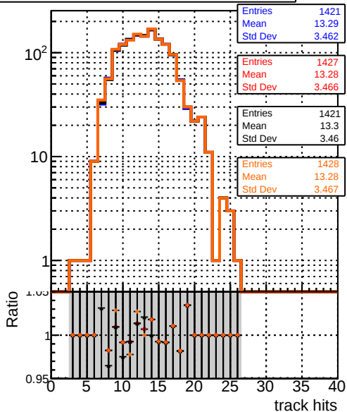
mean hit /data2/legianni/pareto-opt/restart/CMSSW_14_0_5/src/MIV-plot/DQM_TT_original_PU DQM_TT_pLF_pt09_1PU DQM_TT_pLF_pt09_2PU DQM_TT_pLF_pt09_3PU
