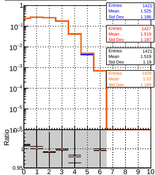
mean hit /data2/legianni/pareto-opt/restart/CMSSW_14_0_5/src/MIV-plot/DQM_TT_original_PU DQM_TT_pLF_pt09_1PU DQM_TT_pLF_pt09_2PU DQM_TT_pLF_pt09_3PU
