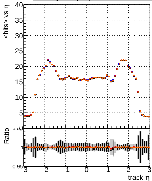
mean hits vs \eta /data2/legianni/pareto-opt/restart/CMSSW_14_0_5/src/MIV-plot/DQM_TT_original_PU DQM_TT pLF pt09_1PU DQM_TT pLF pt09_2PU DQM_TT pLF pt09_3PU
