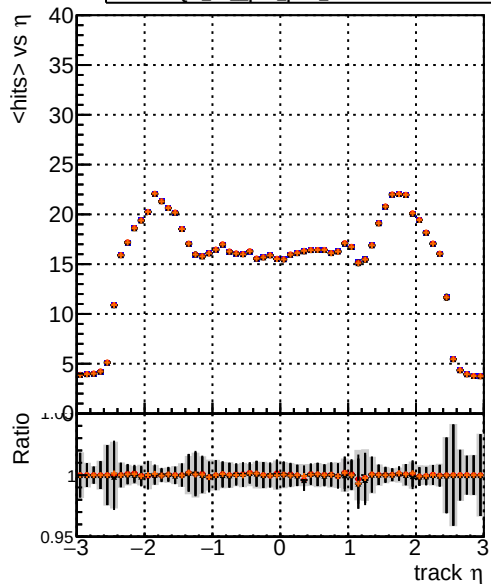
mean hits vs \eta Legend: /data2/legianni/pareto-opt/restart/CMSSW_14_0_5/src/MIV-plot/DQM_TT_original_PU DQM_TT pLF pt09 1PU DQM_TT pLF pt09 2PU DQM_TT pLF pt09 3PU
