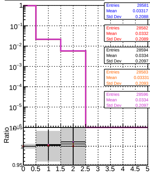
data2/legian/v/pareto-opt/firststart/CMSSW_14_0_5/src/MTV-plot/DQM_TT_original_PU mean hit
