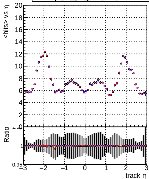
data2/legian/v/pareto-opt/firststart/CMSSW_14_0_5/src/MTV-plot/DQM_TT_original_PU mean hit
