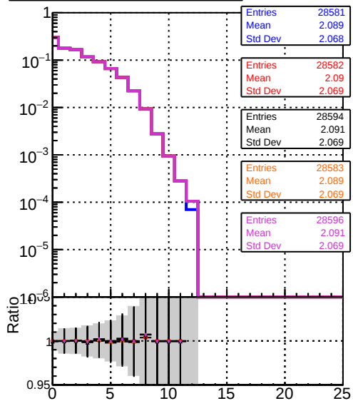
data2/legian/v/pareto-opt/firststart/CMSSW_14_0_5/src/MTV-plot/DQM_TT_original_PU mean hit
