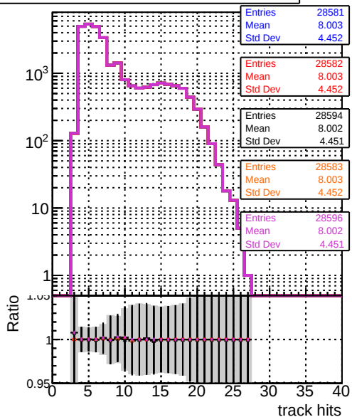
data2/legian/v/pareto-opt/firststart/CMSSW_14_0_5/src/MTV-plot/DQM_TT_original_PU mean hit
