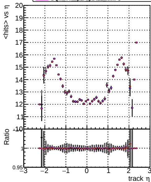
data2legian/tpareto-opt/firststart/CMSSW_14_0_5/src/MTV-plot/DQM_TT_original_PU mean hits DOM TT pLF ptALL z2pPU DOM TT pLF ptALL xxhPU DOM TT pLF ptALL xxhPU
