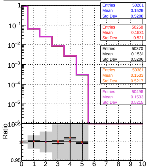
data2legian/tpareto-opt/firststart/CMSSW_14_0_5/src/MTV-plot/DQM_TT_original_PU mean hits DOM TT pLF ptALL z2pPU DOM TT pLF ptALL xxhPU DOM TT pLF ptALL xxhPU
