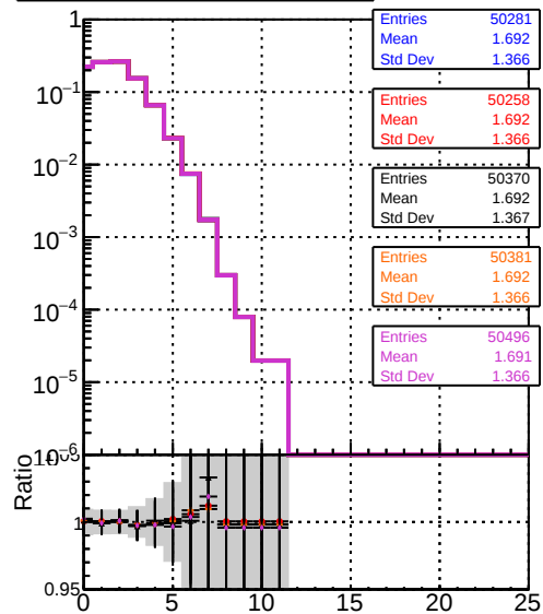
data2legian/tpareto-opt/firststart/CMSSW_14_0_5/src/MTV-plot/DQM_TT_original_PU mean hits DOM TT pLF ptALL z2pPU DOM TT pLF ptALL xxhPU DOM TT pLF ptALL xxhPU
