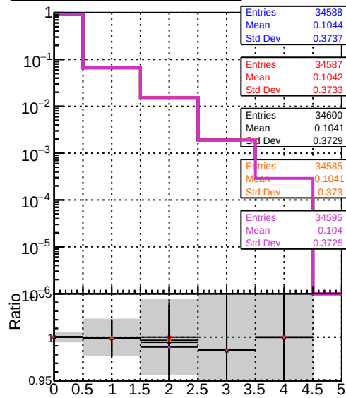
Data2legian/tpareto-opt/Restart/CMSSW_14_0_5/src/MTV-plot/DQM TT original PU
