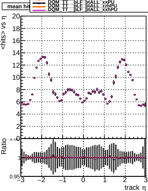
Data2legian/tpareto-opt/Restart/CMSSW_14_0_5/src/MTV-plot/DQM TT original PU
