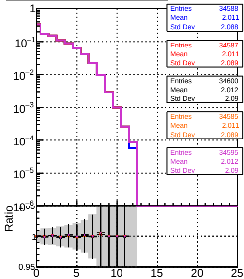
Data2legian/tpareto-opt/Restart/CMSSW_14_0_5/src/MTV-plot/DQM TT original PU
