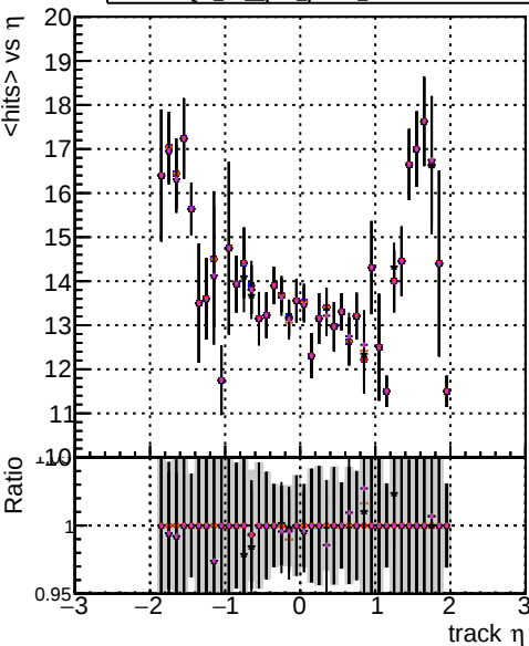
mean hits vs \eta Legend: Data2legion, upareto, opt, restart, CMSSW_14_0_5/src/MTV-plot/DQM_TT_original_PU, DQM_TT, pLF, ptALL, z2p, DQM_TT, pLF, ptALL, xxPU, DQM_TT, pLF, ptALL, zzhPU, DQM_TT, pLF, ptALL, xxhPU
