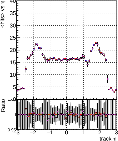
mean hits vs \eta Legend: Data (blue), TT (red), pLF (orange), pTALL (purple), zzhPU (green), xxhPU (brown), and original PU (black).
