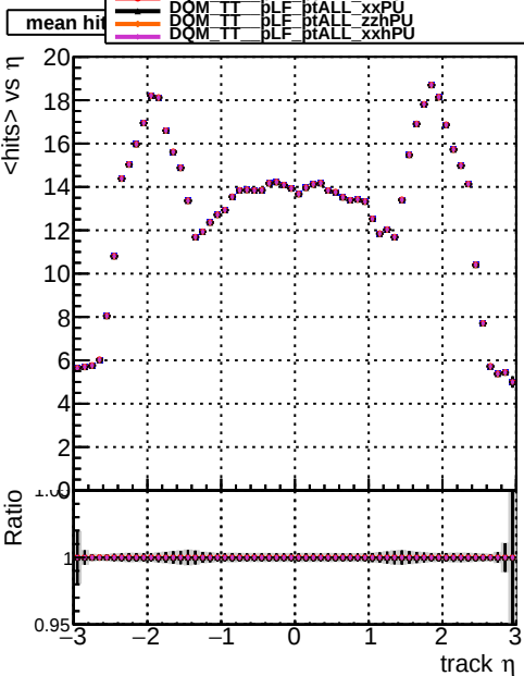
data2legion/tpareto-opt/Restart/CMSSW_14_0_5/src/MTV-plot/DQM_TT_original_PU
