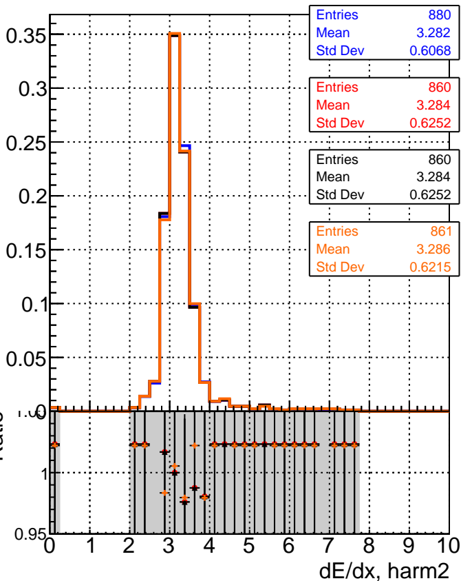
—●— DQM_TT original —●— DQM_TT 0pt09_PU —●— DQM_TT 1pt09_PU —●— DQM_TT 2pt09_PU
