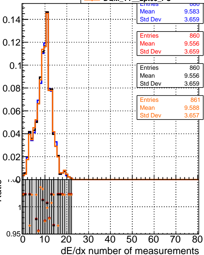
—●— DQM_TT original —●— DQM_TT 0pt09_PU —●— DQM_TT 1pt09_PU —●— DQM_TT 2pt09_PU
