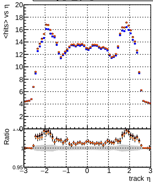
Legend: DQM TT original (blue line), DQM TT 0pt09_PU (red line), DQM TT 1pt09_PU (black line), DQM TT 2pt09_PU (orange line) mean hit
