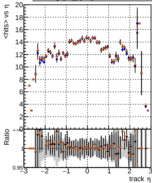
Legend: DQM TT original (blue line), DQM TT 0pt09_PU (red line), DQM TT 1pt09_PU (black line), DQM TT 2pt09_PU (orange line) mean hits
