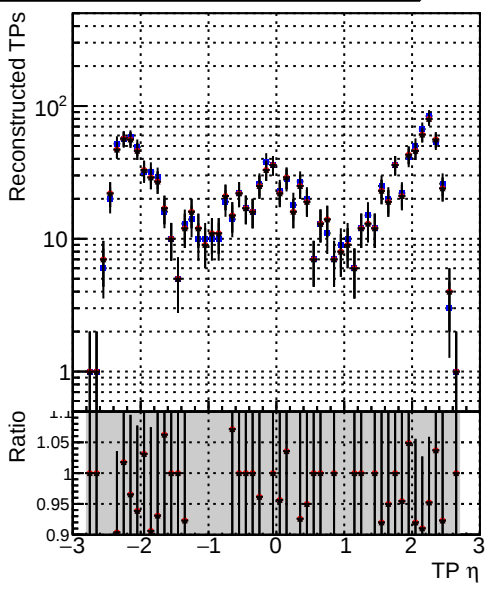
Legend: DQM_TT_original (blue dots), DQM_TT_0pt09_PU3 (red dots), DQM_TT_1pt09_PU3 (black dots)
