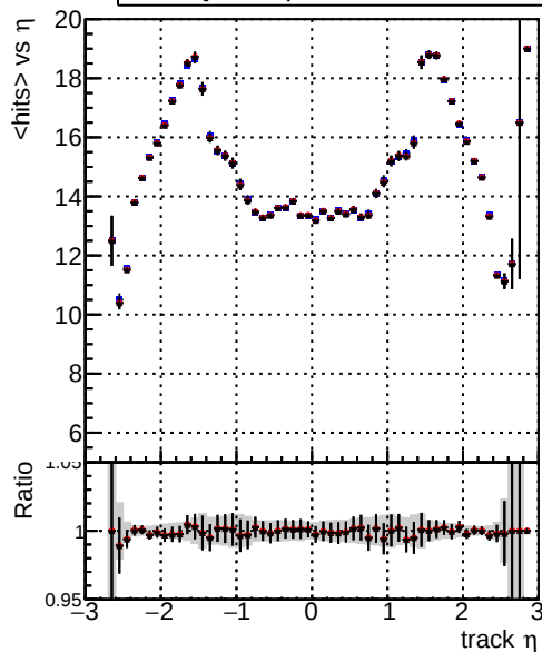
mean hit — DQM_TT_original — DQM_TT_0pt09_PU3 — DQM_TT_1pt09_PU3
