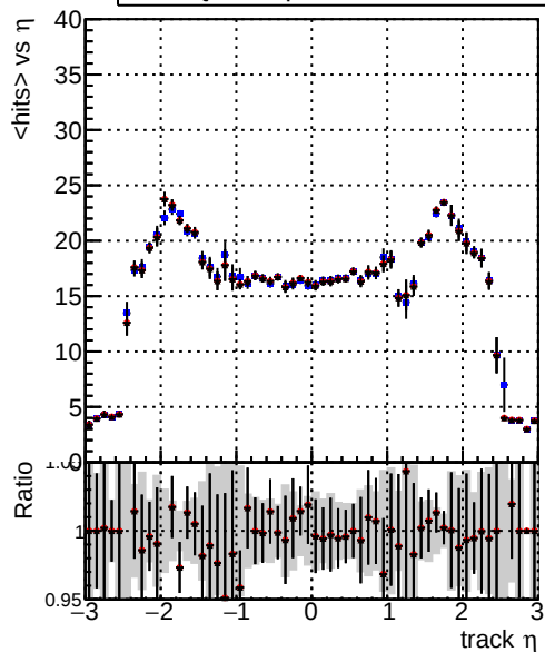
mean hit — DQM_TT_original — DQM_TT_0pt09_PU3 — DQM_TT_1pt09_PU3
