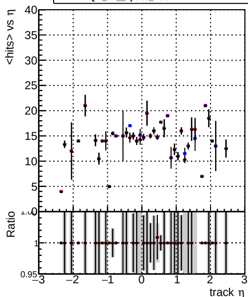
mean hits — DQM_TT_original — DQM_TT_0pt09_PU3 — DQM_TT_1pt09_PU3
