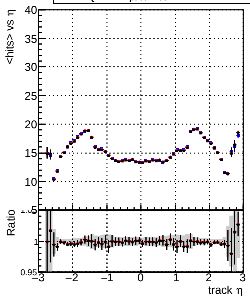
mean hit — DQM_TT_original — DQM_TT_0pt09_PU3 — DQM_TT_1pt09_PU3
