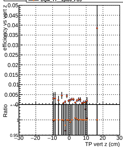
DQM_TT_0pt09_PU3 Efficiend DQM_TT_1pt09_PU3 DQM_TT_2pt09_PU3
