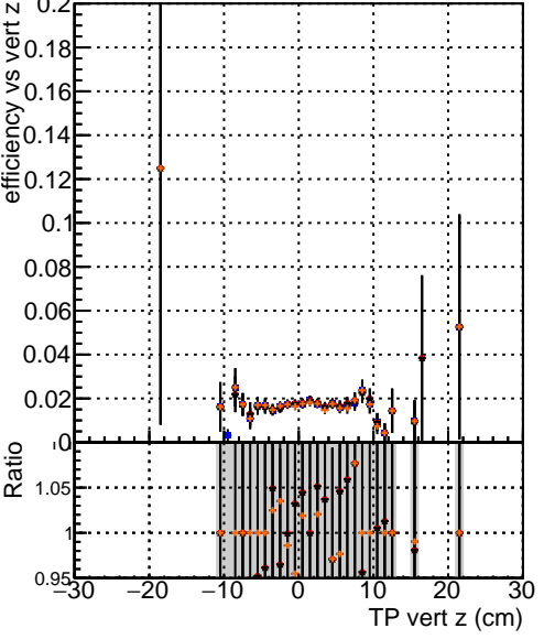
Efficiency vs. sim PV z —●— DQM TT original —●— DQM TT 0pt09_PU3 —●— DQM TT 1pt09_PU3 —●— DQM TT 2pt09_PU3
