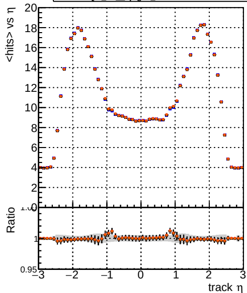
mean hits vs \eta Legend: - DQM TT original (blue line with circles) - DQM TT 0ptg09 PU2 (red line with circles) - DQM TT 1ptg09 PU2 (black line with circles) - DQM TT 2ptg09 PU2 (orange line with circles)
