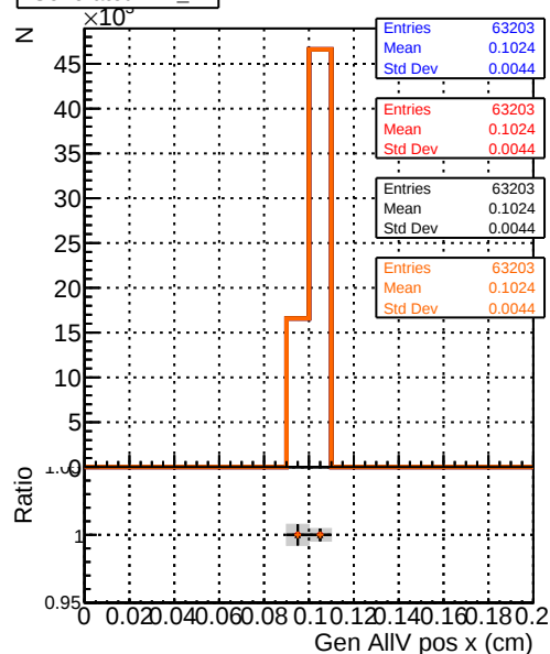
GeneratedTT
