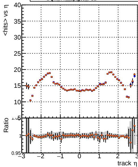
Legend: DQM TT original (blue line), DQM TT 0ptg09 PU2 (red line), DQM TT 1ptg09 PU2 (black line), DQM TT 2ptg09 PU2 (orange line) mean hits
