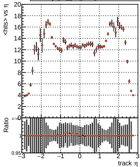
mean hits /data2/legianni/pareto-opt/restart/CMSSW_14_0_5/src/MIV-plot/DQM_TT_original_PU DQM_TT pLB_eta09_1PU DQM_TT pLB_eta09_2PU DQM_TT pLB_eta09_3PU
