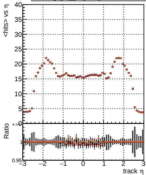
mean hits vs \eta Legend: /data2/legianni/pareto-opt/restart/CMSSW_14_0_5/src/MIV-plot/DQM_TT_original_PU (blue line), DQM_TT_pLB_eta09_1PU (red line with dots), DQM_TT_pLB_eta09_2PU (black line with dots), DQM_TT_pLB_eta09_3PU (orange line with dots)
