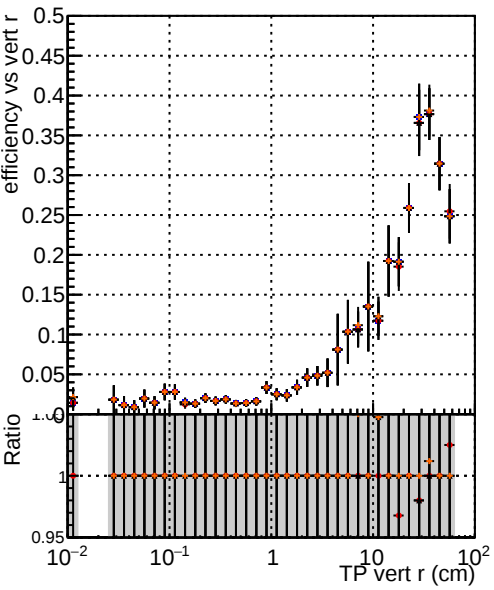
Efficiency vs vertpos Legend: \bullet /data2/legianni/pareto-opt/restart/CMSSW_14_0_5/src/MIV-plot/DQM_TT_original_PU \circ DQM_TT_pLB_eta09_1PU \triangle DQM_TT_pLB_eta09_2PU \square DQM_TT_pLB_eta09_3PU
