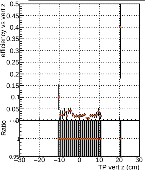
Efficiency vs vertpos Legend: \bullet /data2/legianni/pareto-opt/restart/CMSSW_14_0_5/src/MIV-plot/DQM_TT_original_PU \circ DQM_TT_pLB_eta09_1PU \triangle DQM_TT_pLB_eta09_2PU \square DQM_TT_pLB_eta09_3PU
