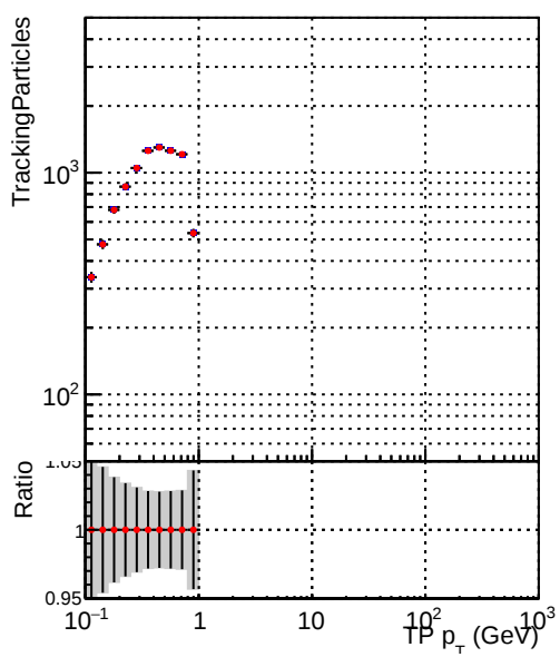
Legend: ● DQM_CKF ● DQM_mkFitnit
