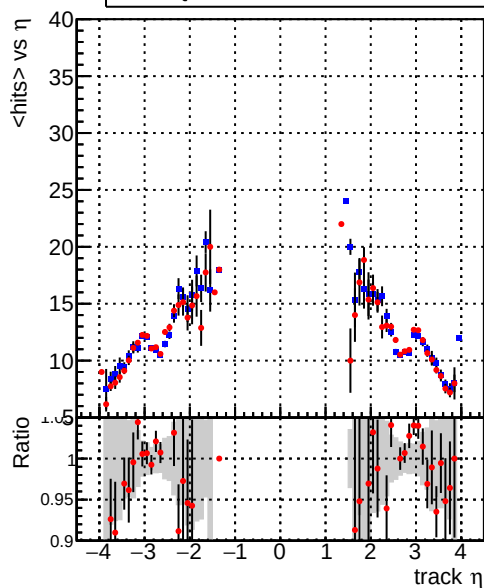
mean hits Legend: DQM_CKF (blue line), DQM_mkFitnit (red line)
