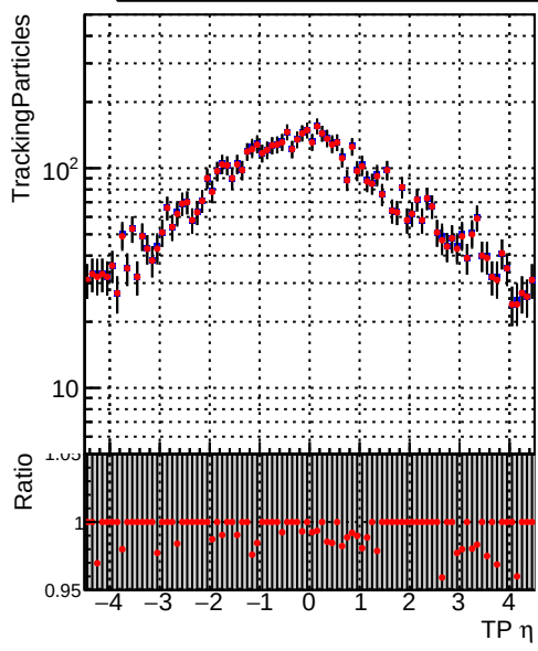
Legend: DQM_CKF (blue dots), DQM_mkFitnit (red dots)
