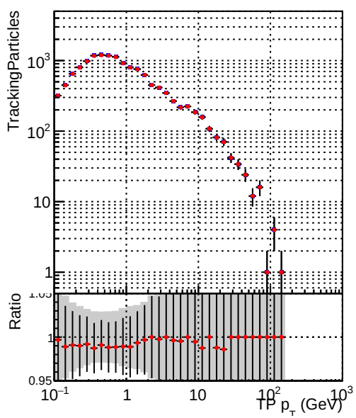
Legend: DQM_CKF (blue dots), DQM_mkFitnit (red dots)
