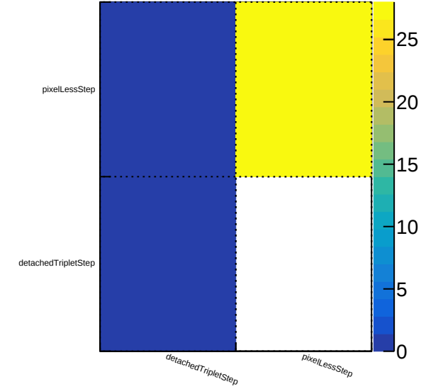
Duplicate tracks: originalAlgo vs originalAlgo
