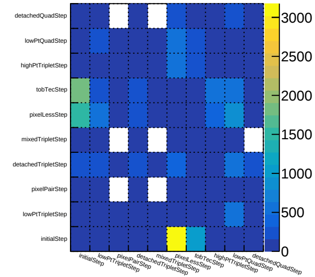
Duplicate tracks: originalAlgo vs originalAlgo
