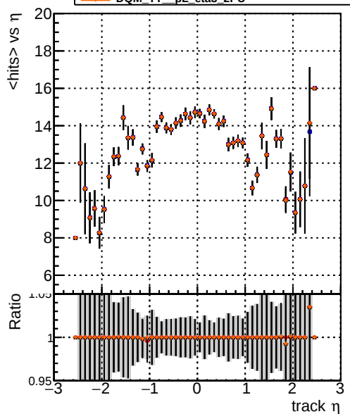
mean hits vs \eta Legend: - blue line: DQM_TT_original PU - red line: DQM_TT_pL_eta3_1PU - black line: DQM_TT_pL_eta3_2PU - orange line: DQM_TT_pL_eta3_2PU
