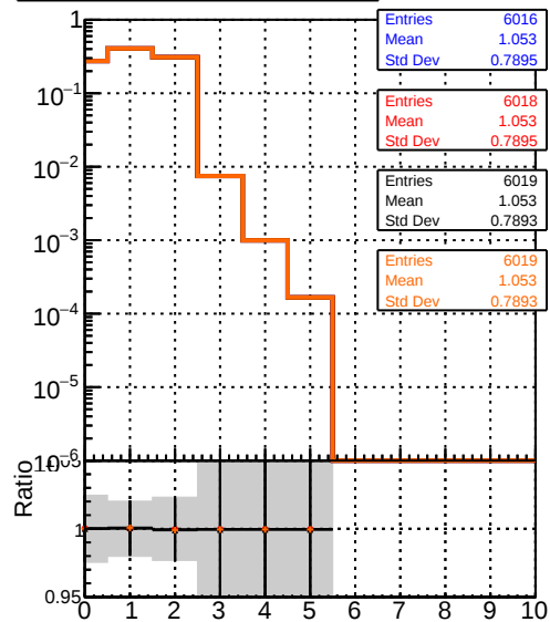
mean hits vs \eta Legend: - blue line: DQM_TT_original PU - red line: DQM_TT_pL_eta3_1PU - black line: DQM_TT_pL_eta3_2PU - orange line: DQM_TT_pL_eta3_2PU
