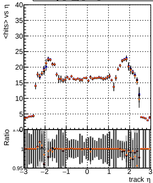
mean hits vs \eta DQM TT original PU DQM TT pf_eta25_1PU DQM TT pf_eta25_2PU DQM TT pf_eta25_3PU
