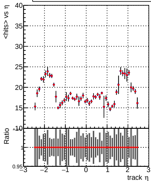
mean hits vs \eta Legend: — DQM_TT_original_noPU — /data2/legianni/pareto-opt/restart/CMSSW_14_0_5/src/MTV-plot/DQM_TT_original_PU
