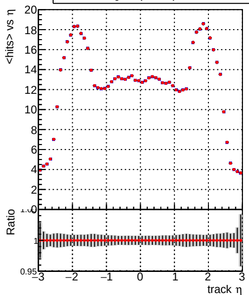
mean hit — DQM_TT__original_noPU — /data2/legianni/pareto-opt/restart/CMSSW_14_0_5/src/MTV-plot/DQM_TT__original_PU
