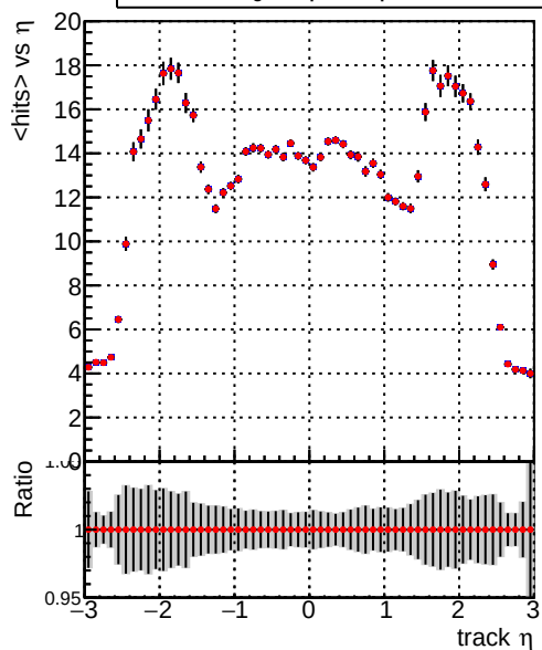
mean hit — DQM_TT__original_noPU — /data2/legianni/pareto-opt/restart/CMSSW_14_0_5/src/MTV-plot/DQM_TT__original_PU
