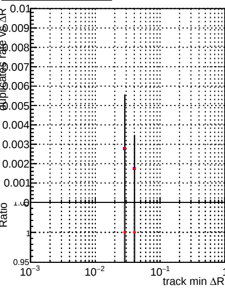
DQM_TT_original_noPU /data2/legianni/pareto-opt/restart/CMSSW_14_0_5/src/MTV-plot/DQM_TT_original_PU
