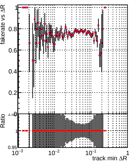
DQM_TT_original_noPU /data2/legianni/pareto-opt/restart/CMSSW_14_0_5/src/MTV-plot/DQM_TT_original_PU
