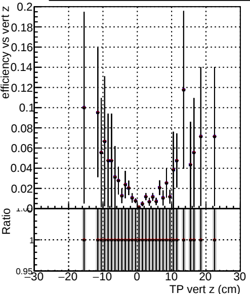
Efficiency vs TP vert z (cm) Legend: DQM_TT_originalREDO100 DQM_TT_originalREDO100f DQM_TT_originalREDO100fb3
