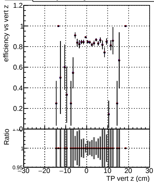
Efficiency vs vert z —●— DQM_TT_originalREDO100 —●— DQM_TT_originalREDO100f —●— DQM_TT_originalREDO100fb3
