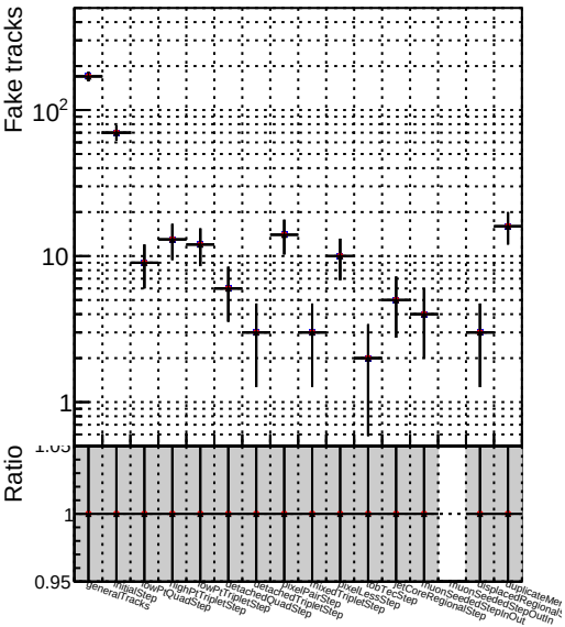
Number Legend ● DQM_TT__originalREDO100f ▲ DQM_TT__originalREDO100fb3
