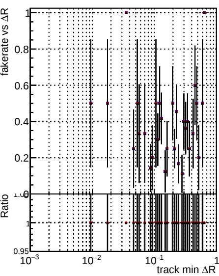
Fake rate vs \Delta R(\text{track, jet}) Legend: DQM TT originalREDO100 (blue dots) DQM TT originalREDO100f (red dots) DQM TT originalREDO100fb3 (black dots)
