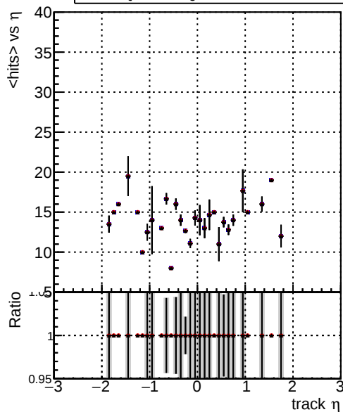
mean hit — DQM_TT_originalREDO100 — DQM_TT_originalREDO100f — DQM_TT_originalREDO100fb3
