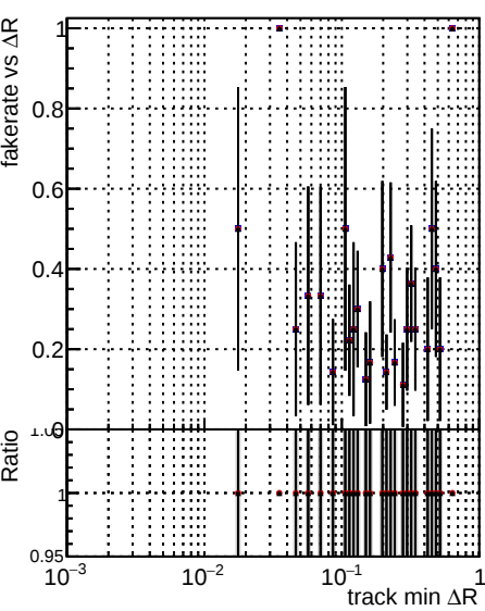
Fake rate vs \Delta R(\text{track, jet}) Legend: DQM TT originalREDO100 (black square) DQM TT originalREDO100f (red circle) DQM TT originalREDO100fb3 (black triangle)
