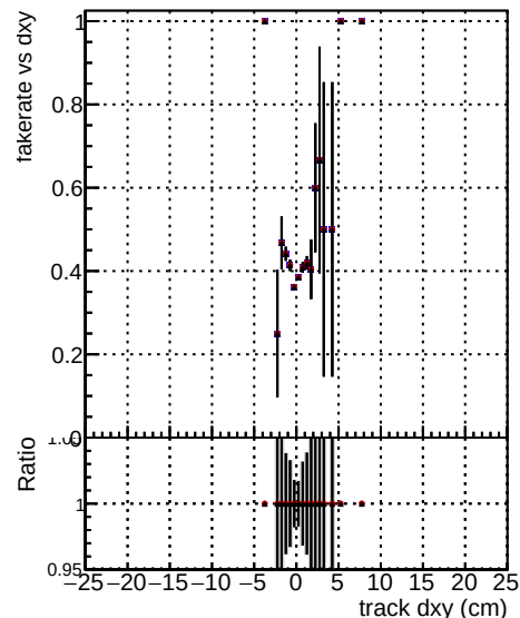
Fake rate vs d DOM TT original REDO100 DOM TT original REDO100f DOM TT original REDO100fb3
