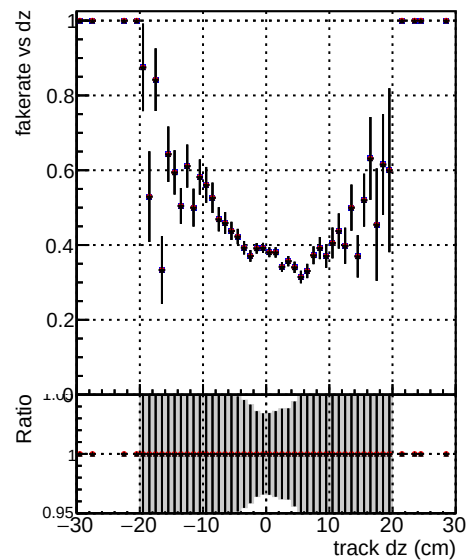
Fake rate vs d DOM TT original REDO100 DOM TT original REDO100f DOM TT original REDO100fb3
